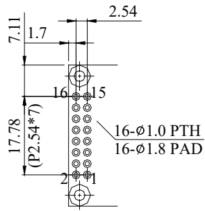
PIN DETAIL
