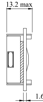
LED B/L
